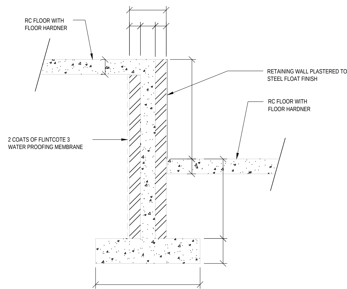
SECTION D (DWG 002) SCALE 1:20
