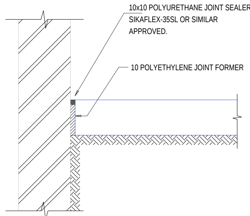
JOINT TYPE A SCALE 1:10
