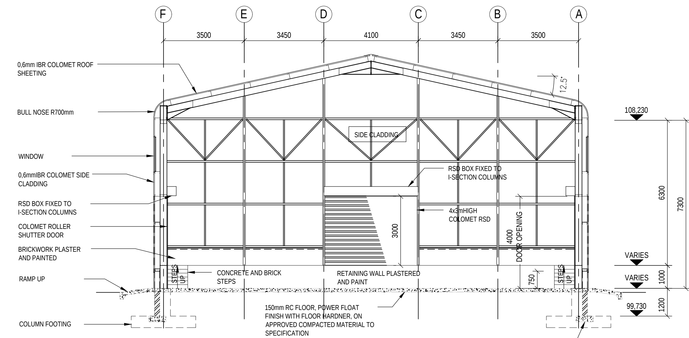
SECTION B-B: BUILDING WORKS (DWG 002) SCALE 1:100
