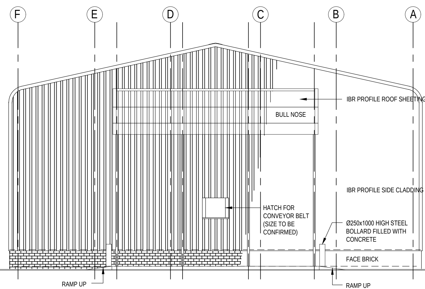
ELEVATION SCALE 1:100
