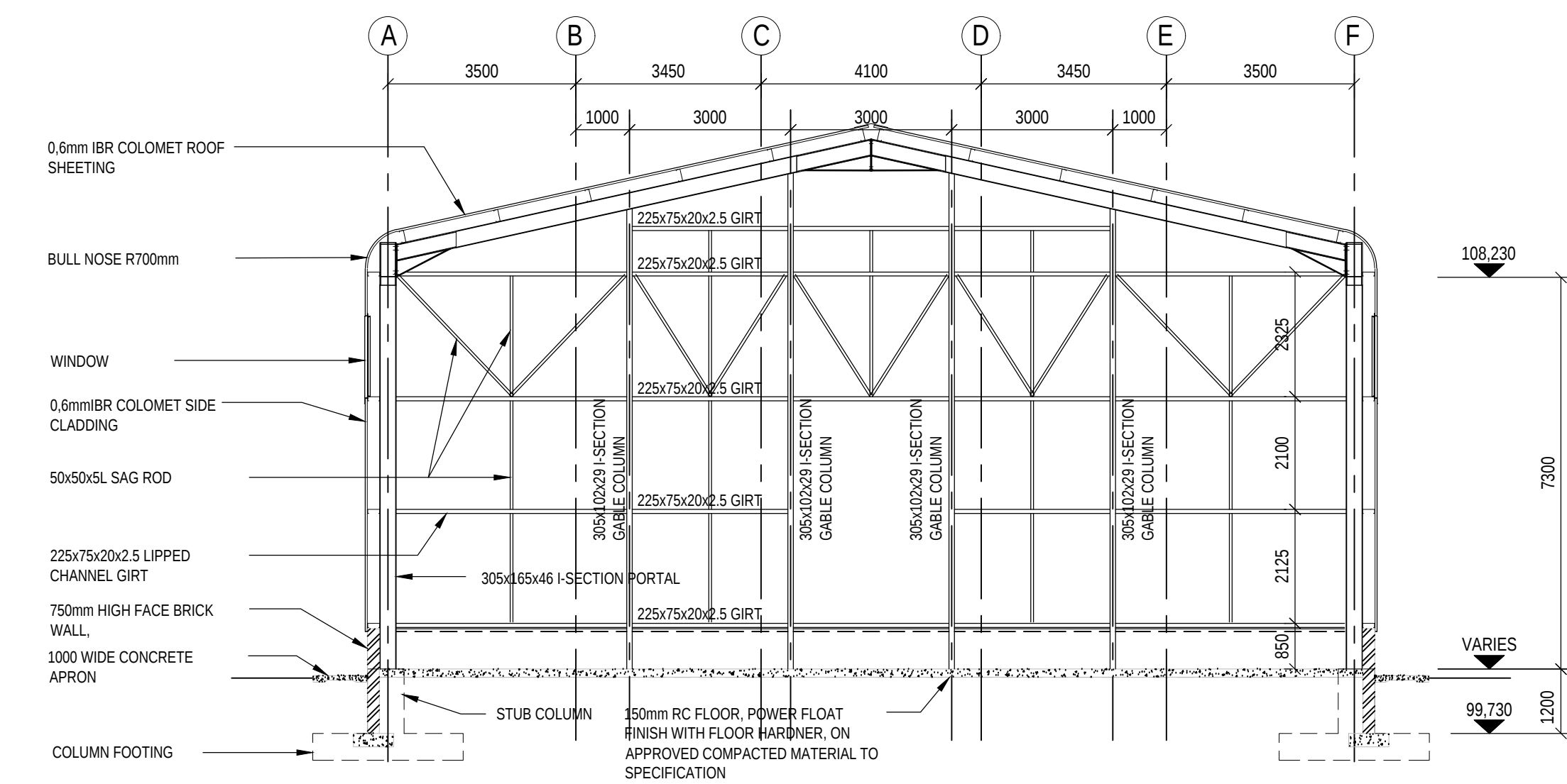
SECTION C-C (DWG 002) SCALE 1:100
