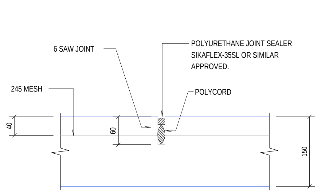
JOINT TYPE B (SAWN JOINT) SCALE 1:10
