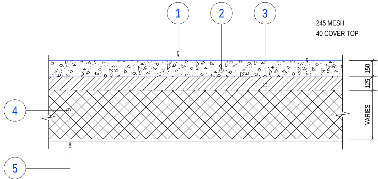
TYPICAL BACKFILL DETAIL
