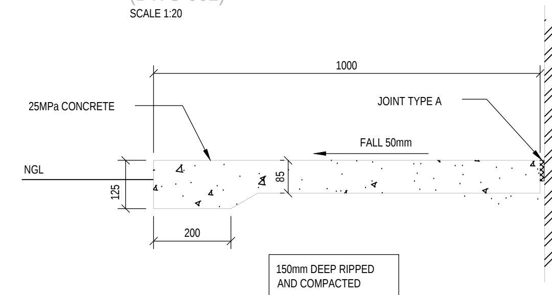
TYPICAL APRON DETAIL SCALE 1:10
