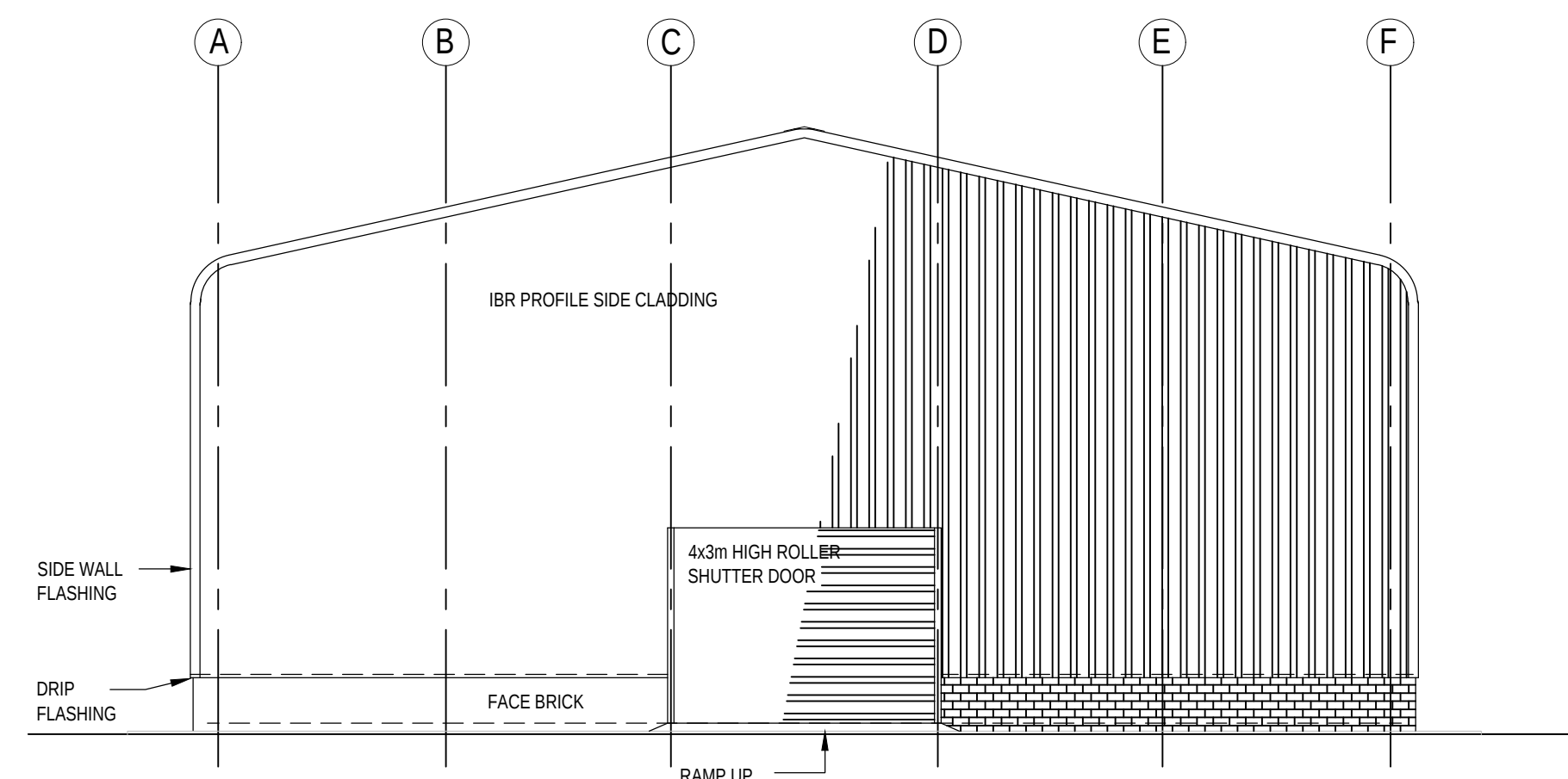
ELEVATION SCALE 1:100
