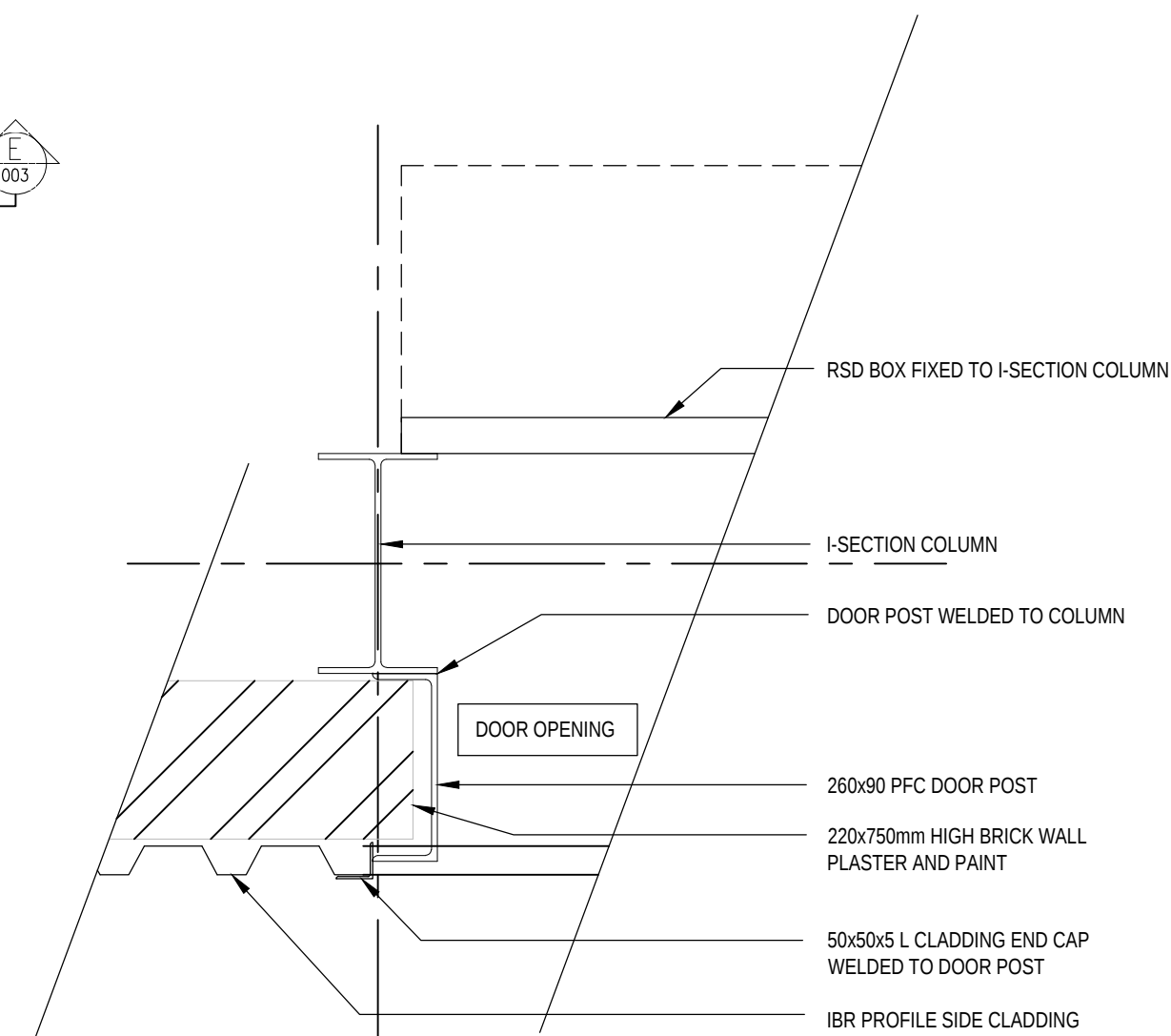
DETAIL 1 (DWG 002) SCALE 1:10
