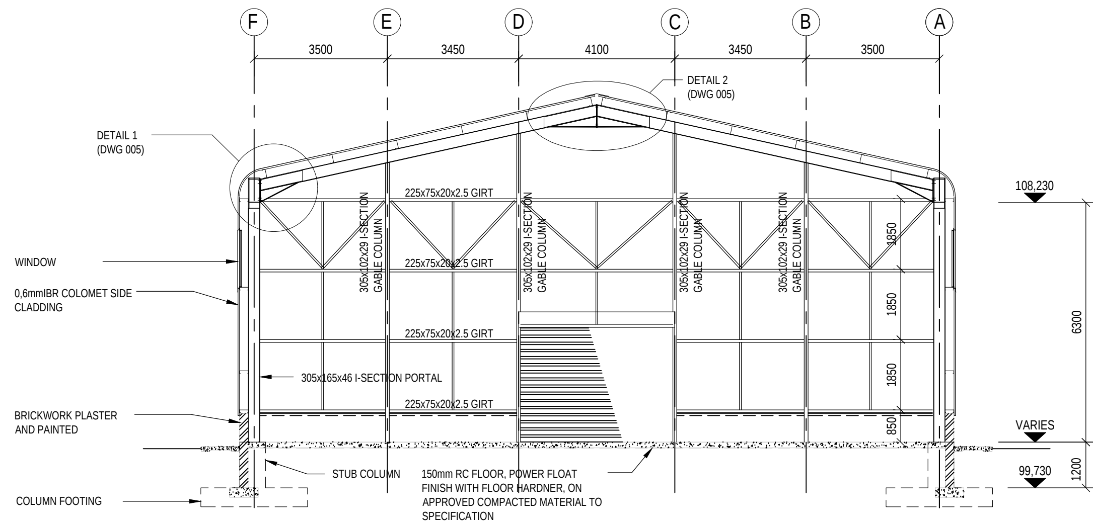
SECTION A-A (DWG 002) SCALE 1:100
