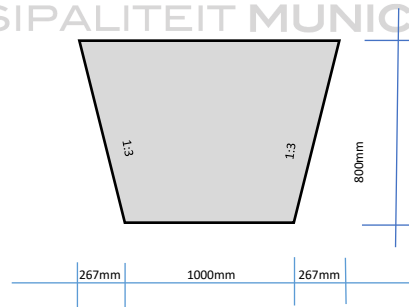
Figure 2: Open Channel Cross Section (stone pitch)
