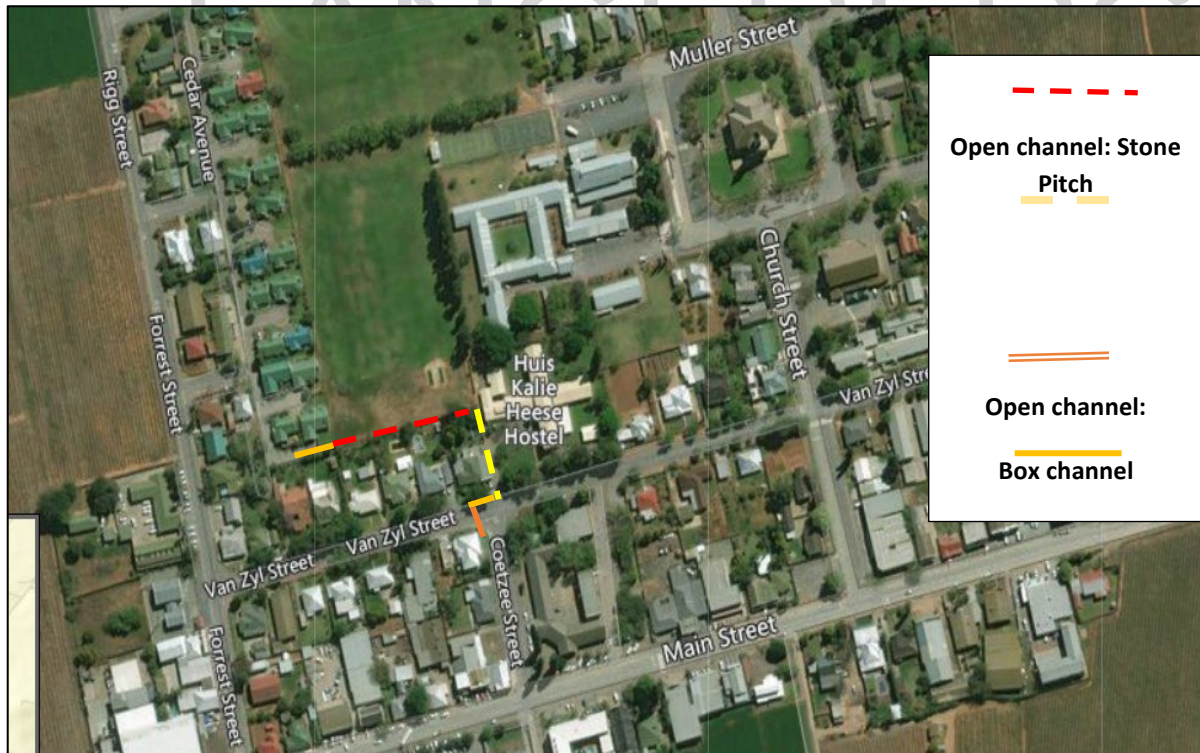
Figure 1: Locality Plan with proposed diversion
