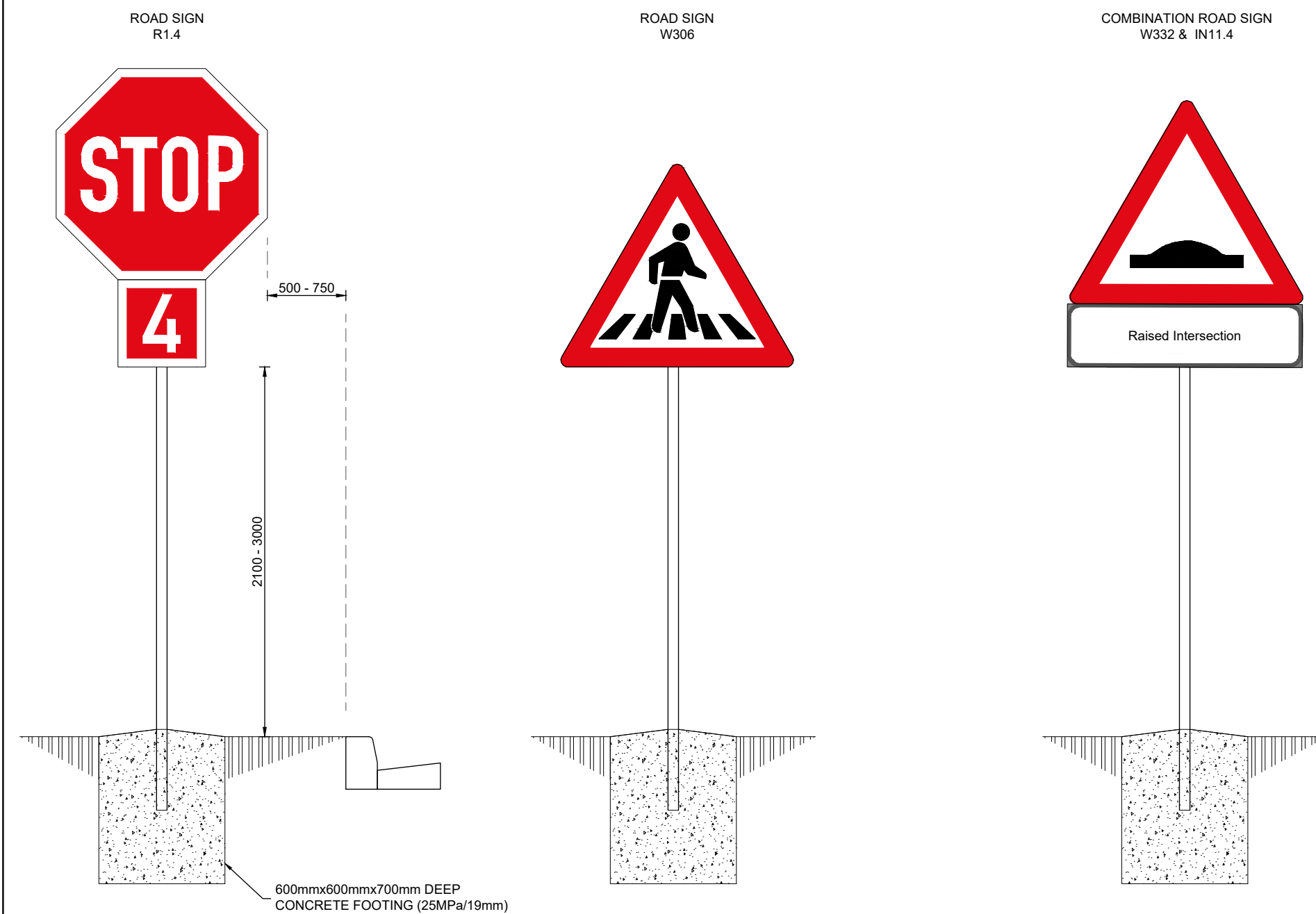
TYPICAL ROAD SIGNS SCALE 1:50
