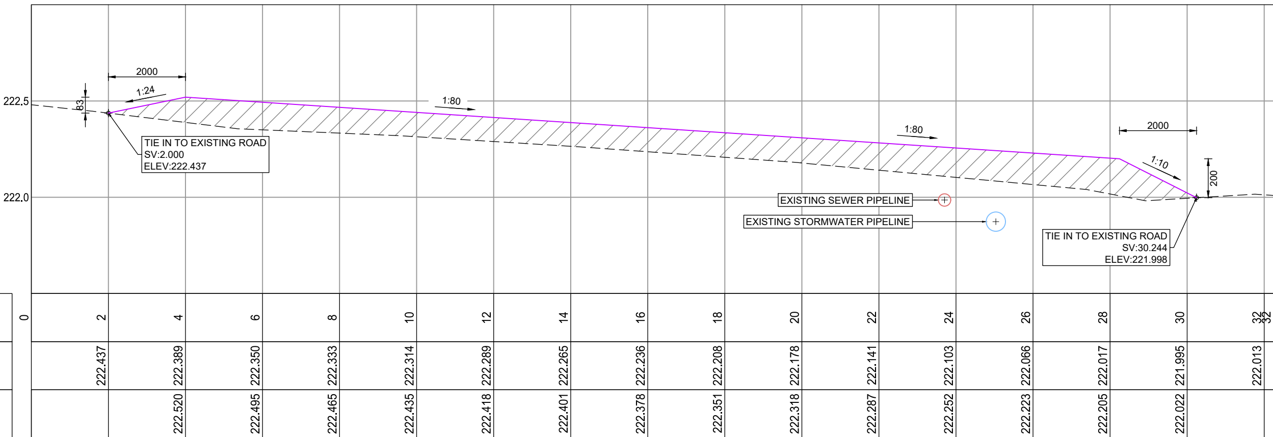
LONGITUDINAL SECTION - CROSS ROAD
