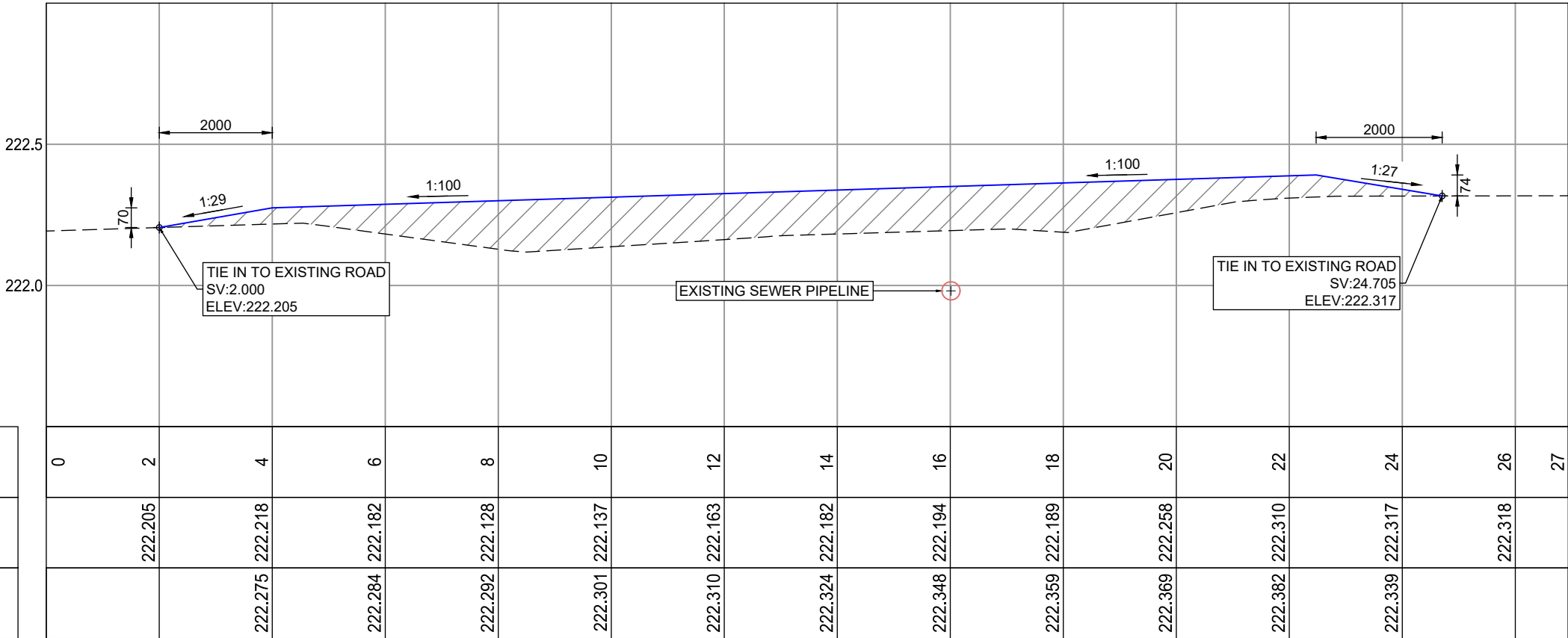
LONGITUDINAL SECTION - BATH ROAD
