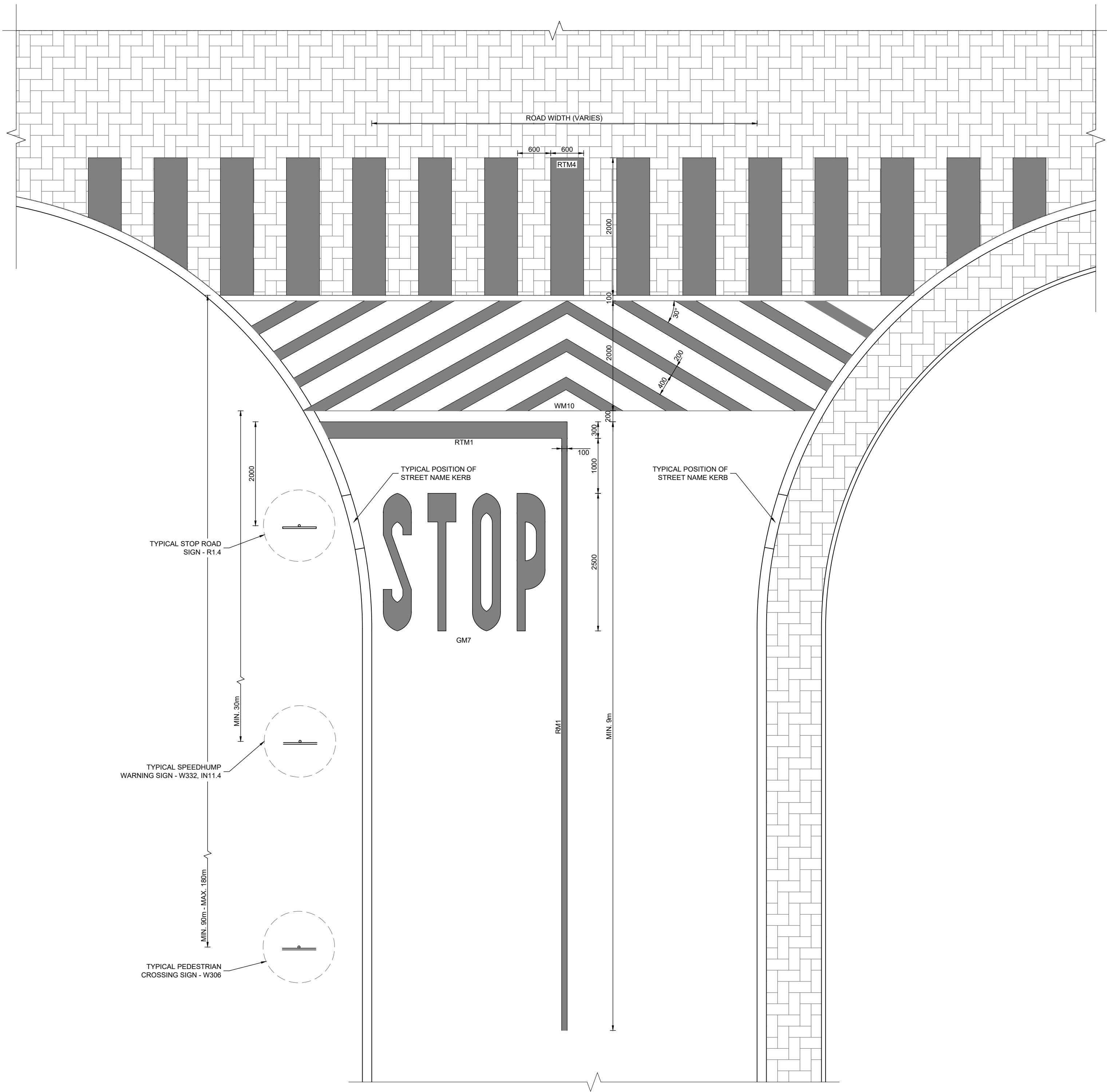
TYPICAL INTERSECTION ROAD MARKINGS SCALE 1:50
