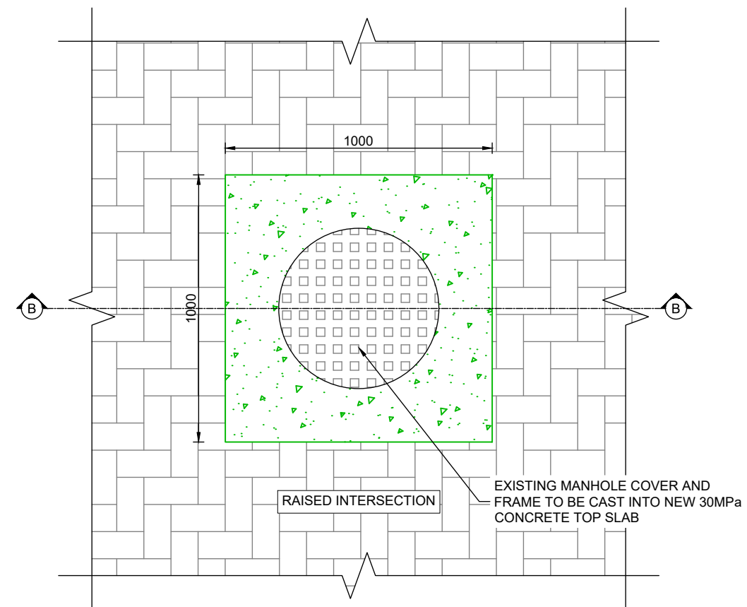
MANHOLE CONCRETE TOP SLAB PLAN VIEW
