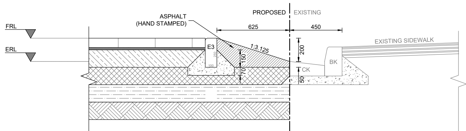
SECTION B-B SCALE 1:20
