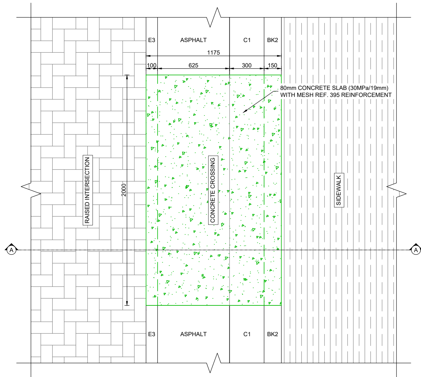
PEDESTRIAN CROSSING PLAN VIEW
